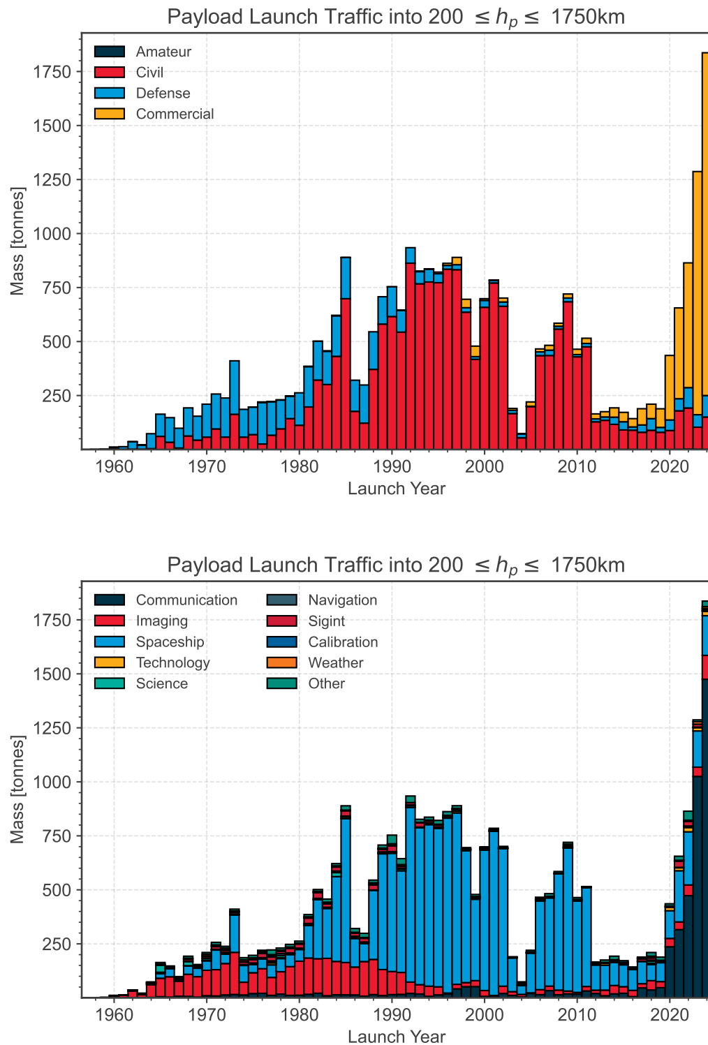
Figure 2.13: Evolution of the launch traffic near \text{LEO}_{\text{IADC}} per mission funding (top) and type (bottom) in terms of mass.
