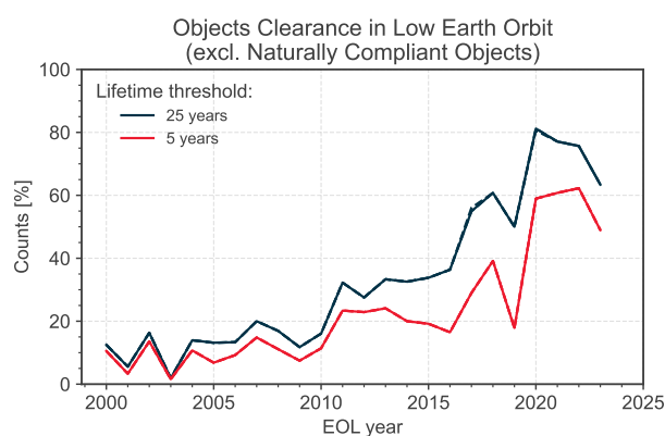
(d) Relative clearance near LEO_{IADC} by payloads and rocket bodies for 25 and 5-year lifetime limits.
