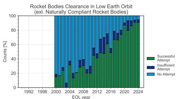
(b) Relative clearance of LEO_{IADC} by rocket bodies, for a lifetime limit of 25 years.
